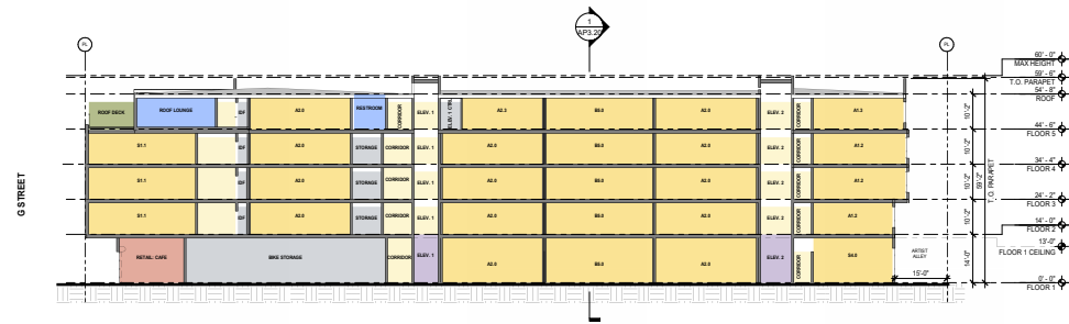
BUILDING SECTION - SHORT 1.0 2 1/16" = 1'-0"
